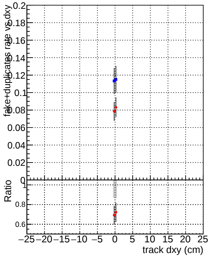
DQM_V0001_R000000001_Global_CMSSW_ckfnocut2_RECO DQM_V0001_R000000001_Global_CMSSW_mknocut2_RECO
