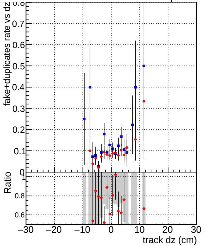
DQM_V0001_R000000001_Global_CMSSW_ckfnocut2_RECO DQM_V0001_R000000001_Global_CMSSW_mknocut2_RECO
