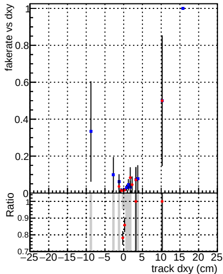
—●— DQM V0001_R0000000001 Global CMSSW_ckptnocut2 RECO —●— DQM V0001_R0000000001 Global CMSSW_mknocut2 RECO
