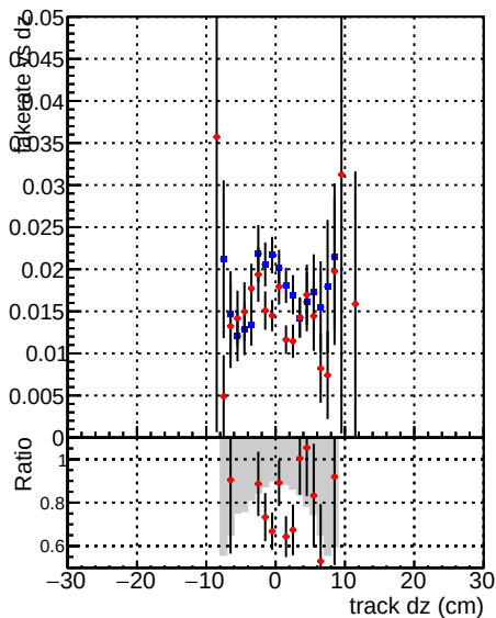
Legend Global CMSSW_ckptnocut2 RECO Fake rate vs d Blue dots DQM V0001_R0000000001 Global CMSSW_ckptnocut2 Red dots DQM V0001_R0000000001 Global CMSSW_mknocut2
