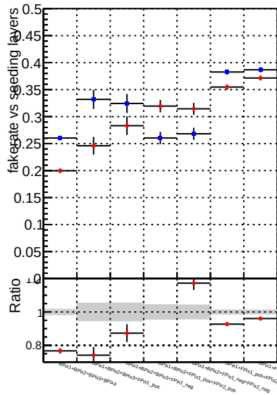
Fake rate vs. DQM V0001_R000000001 Global CMSSW_ckfnocut2 RECO DQM V0001_R000000001 Global CMSSW_mknocut2 RECO
