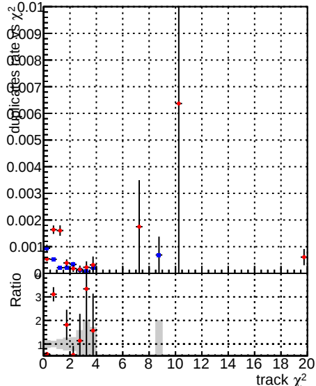
—●— DQM_V0001_R000000001_Global_CMSSW_ckfnocut2_RECO —●— DQM_V0001_R000000001_Global_CMSSW_mknocut2_RECO
