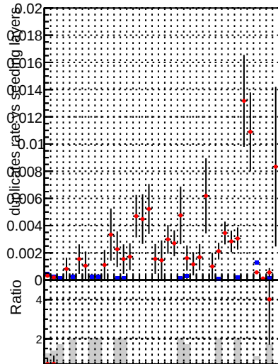
—●— DQM_V0001_R000000001_Global_CMSSW_ckfnocut2_RECO —●— DQM_V0001_R000000001_Global_CMSSW_mknocut2_RECO
