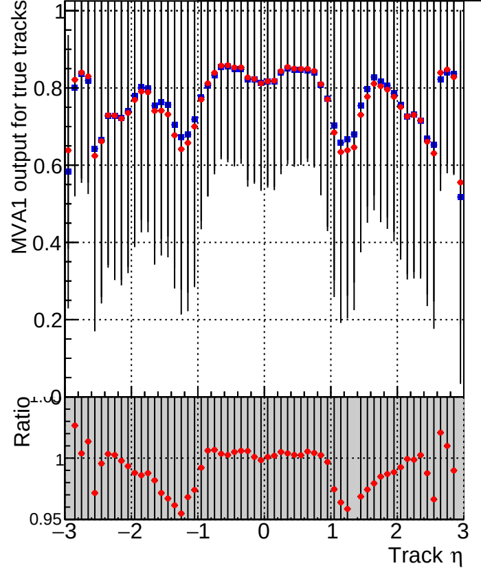
MVA1 of associated tracks (recoToSim) vs. track \eta Legend: \text{DQM\_V0001\_R000000001\_Global\_CMSSW\_ckfnocut2\_RECO} (blue stars) \text{DQM\_V0001\_R000000001\_Global\_CMSSW\_mknocut2\_RECO} (red stars)
