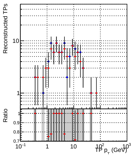
Legend: DQM_V0001_R000000001_Global_CMSSW_cknucut2_RECO (blue line), DQM_V0001_R000000001_Global_CMSSW_mknucut2_RECO (red line)
