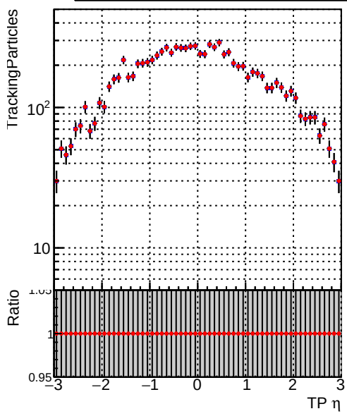
Legend: DQM_V0001_R000000001_Global_CMSSW_cknucut2_RECO (blue line), DQM_V0001_R000000001_Global_CMSSW_mknucut2_RECO (red line)
