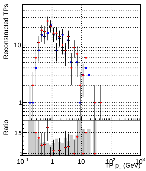
Legend: — DQM_V0001_R000000001_Global_CMSSW_cknocut2_RECO (blue diamonds) — DQM_V0001_R000000001_Global_CMSSW_mknocut2_RECO (red diamonds)
