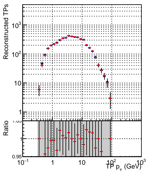
Legend: DQM_V0001_R000000001_Global_CMSSW_ckfnocut2_RECO (blue line), DQM_V0001_R000000001_Global_CMSSW_mknocut2_RECO (red line)
