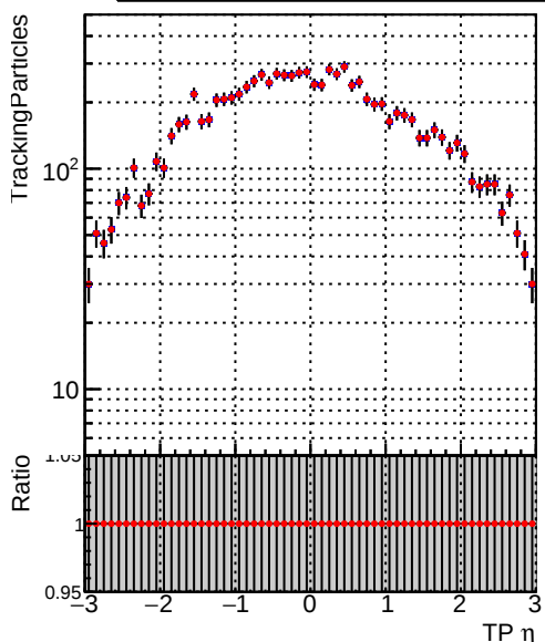
—•— DQM_V0001_R000000001_Global_CMSSW_cknocut2_RECO —•— DQM_V0001_R000000001_Global_CMSSW_mknocut2_RECO
