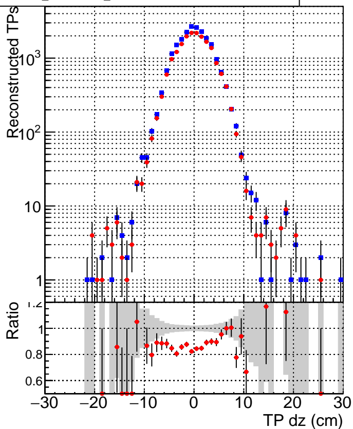
■ DQM_V0001_R000000001_Global_CMSSW_ckfnocut2_RECO ● DQM_V0001_R000000001_Global_CMSSW_mknocut2_RECO
