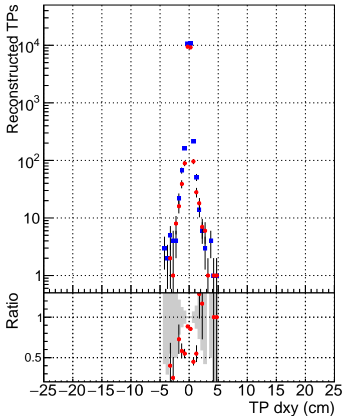
■ DQM_V0001_R000000001_Global_CMSSW_ckfnocut2_RECO ● DQM_V0001_R000000001_Global_CMSSW_mknocut2_RECO
