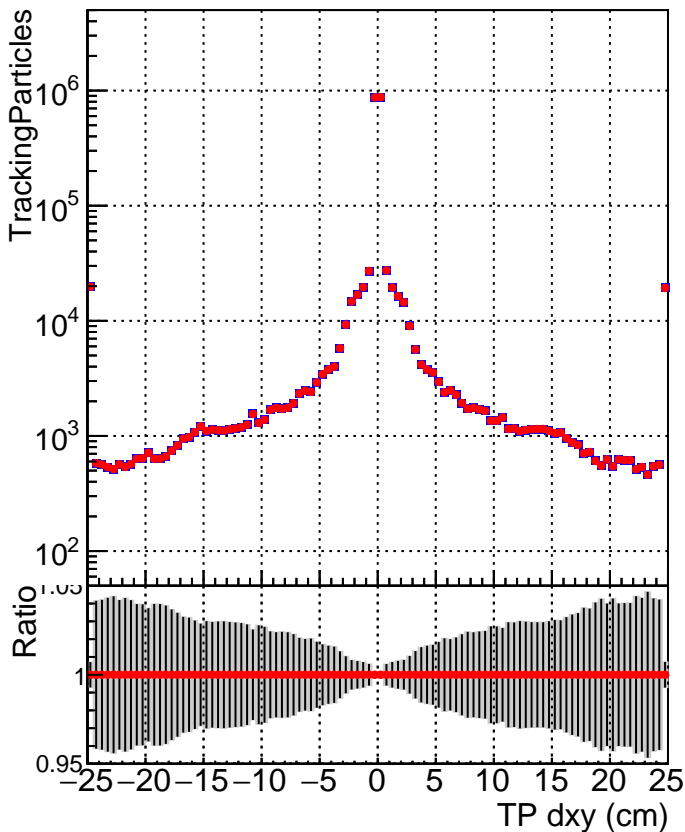
■ DQM_V0001_R000000001_Global_CMSSW_ckfnocut2_RECO ● DQM_V0001_R000000001_Global_CMSSW_mknocut2_RECO
