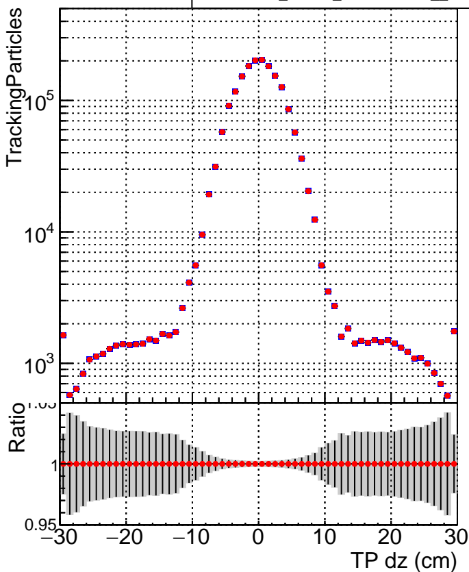
■ DQM_V0001_R000000001_Global_CMSSW_ckfnocut2_RECO ● DQM_V0001_R000000001_Global_CMSSW_mknocut2_RECO
