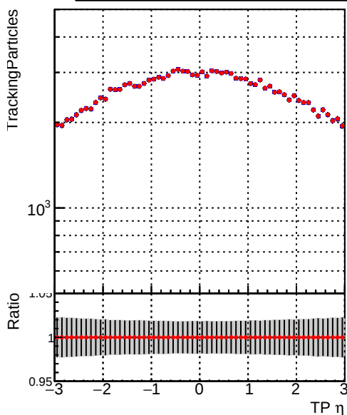
—•— DQM_V0001_R000000001_Global_CMSSW_cknocut2_RECO —•— DQM_V0001_R000000001_Global_CMSSW_mknocut2_RECO
