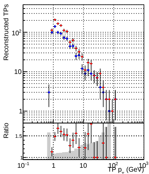
—•— DQM_V0001_R000000001_Global_CMSSW_cknocut2_RECO —•— DQM_V0001_R000000001_Global_CMSSW_mknocut2_RECO
