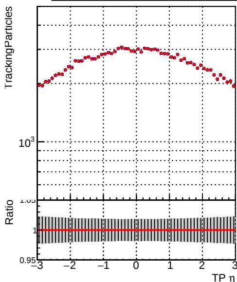
■ DQM_V0001_R0000000001_Global_CMSSW_cknocut2_RECO ■ DQM_V0001_R0000000001_Global_CMSSW_mknocut2_RECO
