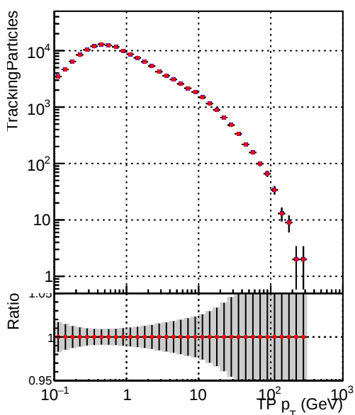
■ DQM_V0001_R0000000001_Global_CMSSW_cknocut2_RECO ■ DQM_V0001_R0000000001_Global_CMSSW_mknocut2_RECO
