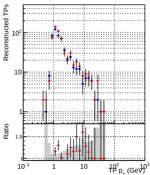
■ DQM_V0001_R0000000001_Global_CMSSW_cknocut2_RECO ■ DQM_V0001_R0000000001_Global_CMSSW_mknocut2_RECO
