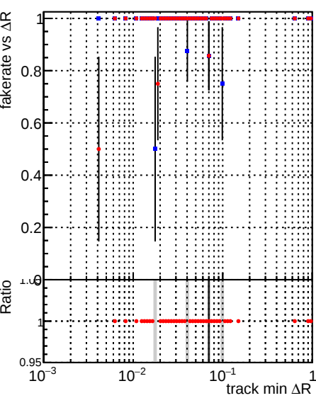
Fake rate vs \Delta R(\text{track, jet}) DQM_V0001_R000000001_Global_CMSSW_ckfnocut2_RECO DQM_V0001_R000000001_Global_CMSSW_mknocut2_RECO
