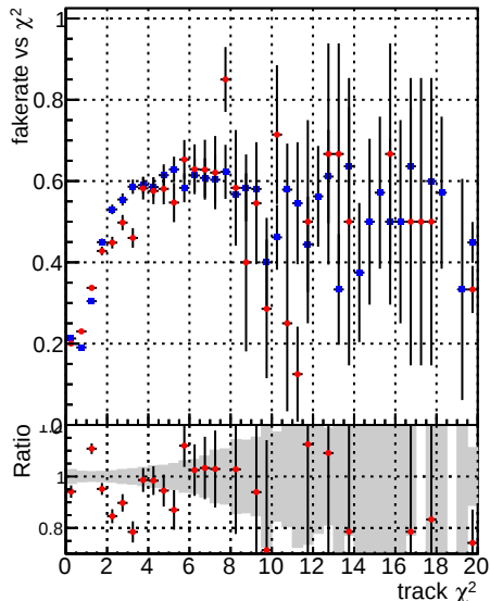
Fake rate vs. —●— DQM V0001_R000000001 Global CMSSW_ckfnocut2 RECO —●— DQM V0001_R000000001 Global CMSSW_mknocut2 RECO
