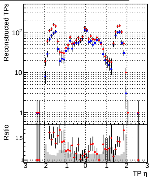
—•— DQM_V0001_R000000001_Global_CMSSW_cknocut2_RECO —•— DQM_V0001_R000000001_Global_CMSSW_mknocut2_RECO
