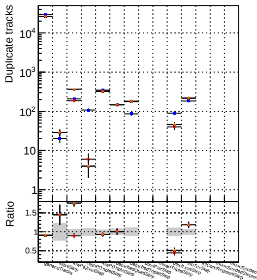
Number of tracks vs collection Legend: DQM_V0001_R000000001_Global_CMSSW_ckptPU50_RECO DQM_V0001_R000000001_Global_CMSSW_mkFitPU50LowPtQuad_RECO DQM_V0001_R000000001_Global_CMSSW_scm05_RECO DQM_V0001_R000000001_Global_CMSSW_scm05+dup_RECO
