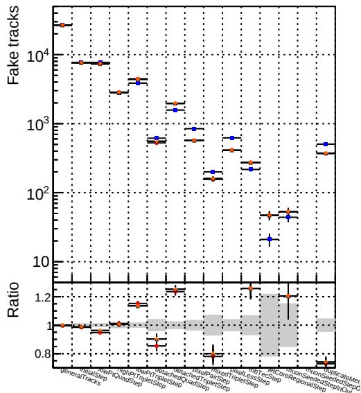
Number of tracks • DQM_V0001_R0000000001_Global_CMSSW_ckptPU50_RECO Number of true tracks • DQM_V0001_R0000000001_Global_CMSSW_mkFitPU50LowPtQuad_RECO Number of fake tracks • DQM_V0001_R0000000001_Global_CMSSW_scmod05_RECO Number of duplicate tracks • DQM_V0001_R0000000001_Global_CMSSW_scmod05+dup_RECO
