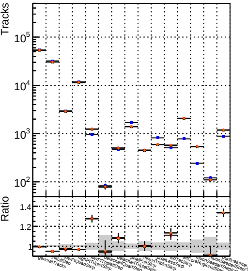
Number Color Label Model Method DOM V0001 Blue R0000000001 Global CMSSW_ktPPU50_RECO DOM V0001 Red R0000000001 Global CMSSW_mkFitPU50LowPQuad_RECO DOM V0001 Green R0000000001 Global CMSSW_scm05_RECO DOM V0001 Black R0000000001 Global CMSSW_scm05+dup_RECO
