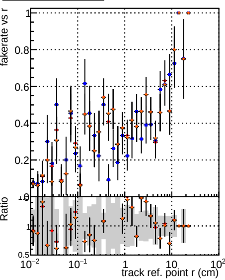
Fake rate vs v Global CMSSW chp50 RECO Global CMSSW chp50 RECO Global CMSSW chp50 RECO Global CMSSW chp50 RECO
