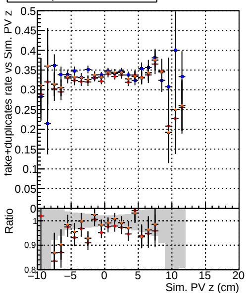
fake+duplicates vs track ref. point r (cm)
