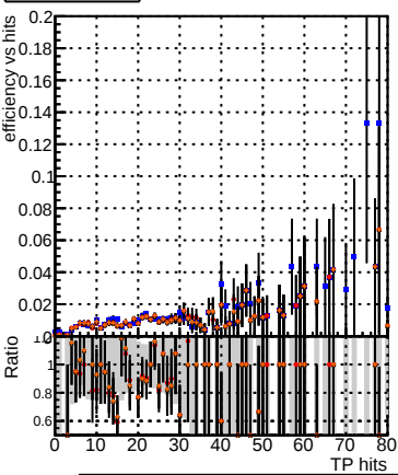
Efficiency vs hit Legend: DQM_V0001_R000000001_Global_CMSSW_ckfPU50_RECO DQM_V0001_R000000001_Global_CMSSW_mkFitPU50LowPtQuad_RECO DQM_V0001_R000000001_Global_CMSSW_scm05_RECO DQM_V0001_R000000001_Global_CMSSW_scm05+dup_RECO
