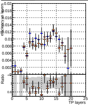
Efficiency vs hit Legend: DQM_V0001_R000000001_Global_CMSSW_ckfPU50_RECO DQM_V0001_R000000001_Global_CMSSW_mkFitPU50LowPtQuad_RECO DQM_V0001_R000000001_Global_CMSSW_scm05_RECO DQM_V0001_R000000001_Global_CMSSW_scm05+dup_RECO
