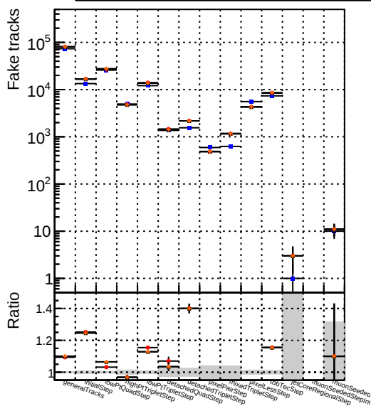
Number DQM_V0001_R000000001 Global CMSSW_ckptPU50_RECO DQM_V0001_R000000001 Global CMSSW_mkFitPU50LowPtQuad_RECO DQM_V0001_R000000001 Global CMSSW_scm0d05_RECO DQM_V0001_R000000001 Global CMSSW_scmod05+dupd RECO
