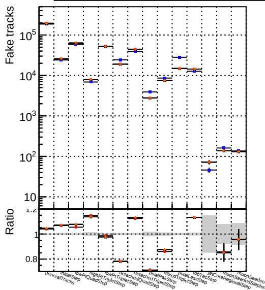
Number Symbol QIM V0001 R0000000001 Global CMSSW ilrFltPUSLOWP+Quau RECO ● QIM V0001 R0000000001 Global CMSSW scmod05 RECO ★ QIM V0001 R0000000001 Global CMSSW scmod05+dup RECO ● QIM V0001 R0000000001 Global CMSSW scmod05+dup RECO
