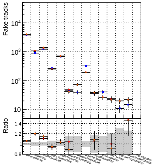
Number ★ DQM_V0001 R000000001 Global CMSSW scmod05_RECO ★ DQM_V0001 R000000001 Global CMSSW scmod05+dup_RECO
