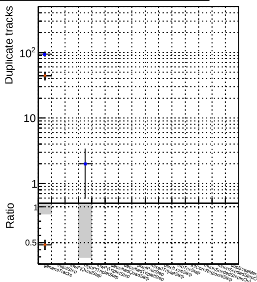
Numbe DQM_V0001 R0000000001 Global CMSSW_mkFitPU50LowPTrQuad_RECO DQM_V0001 R0000000001 Global CMSSW_scmod05_RECO DQM_V0001 R0000000001 Global CMSSW_scmod05+dup_RECO
