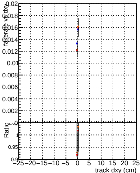
Fake rate vs d DOM V0001 D0000000000001 Global CMSSW skfPH50-RECO 1 DOM V0001 D0000000000001 Global TTWW skfPH50+150-pTQuad_RECO 2 DOM V0001 R0000000000001 Global CMSSW sch08005+800 RECO
