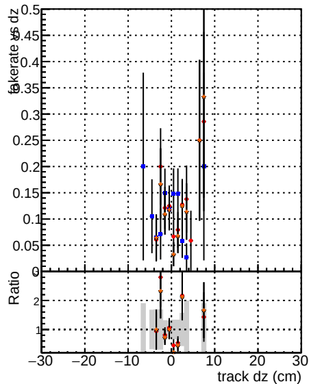
Fake rate vs d DOM V0001 D00000000001 Global CMSSW skPH50-RECO DOM V0001 D00000000001 Global TTWW skPH50+150-pTQuad RECO DOM V0001 R000000000001 Global CMSSW sch08005+800 RECO
