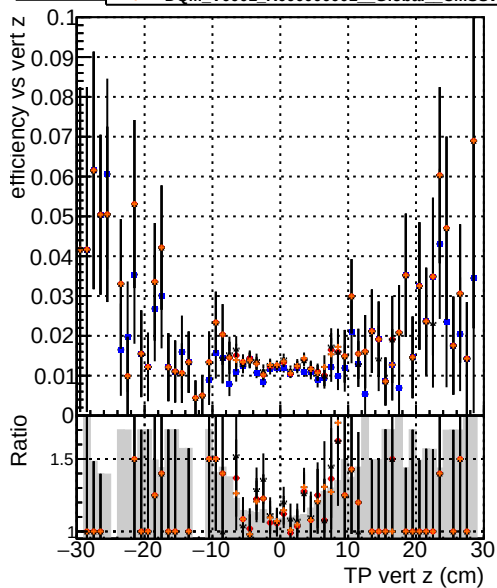
Efficiency Model Dataset Model Model Model Model 0.95 DQM V0001 R0000000001 Global CMSSW mkFitPU50 RECO 0.90 DQM V0001 R0000000001 Global CMSSW mkFitPU50LowPtQuad RECO 0.85 DQM V0001 R0000000001 Global CMSSW mkFitPU50LowPtTriplet RECO
