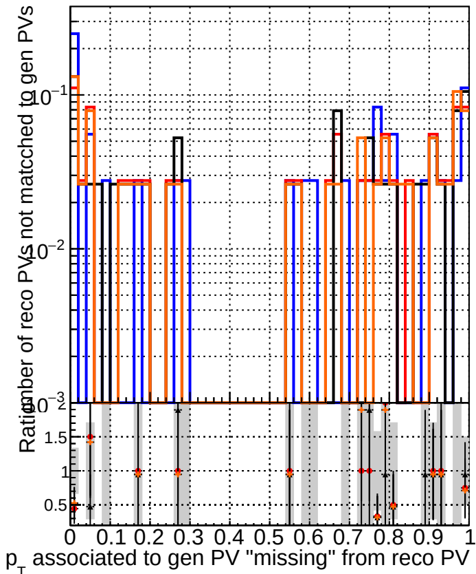
MSSW_MKFitF030E0WFTriplet_REC0 REC0VASSOCZGenPVNotMatched_Missing
