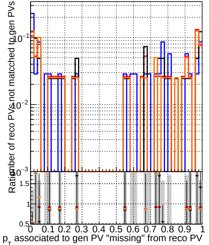
RecoPVAssoc2GenPVNotMatched_missing
