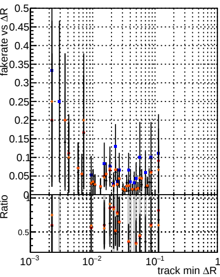
Fake rate vs \Delta R(\text{track, jet}) DQM V00001 R00000000001 Global CMSSW chfPU50 RECO Global CMSSW mktPU50 RECO Global CMSSW mktPU50 LowPQuad RECO Global CMSSW mktPU50 LowPTriplet RECO
