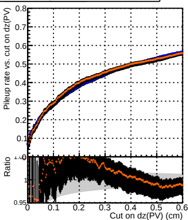
Pileup rate vs. cut on dz(PV) (cm)
