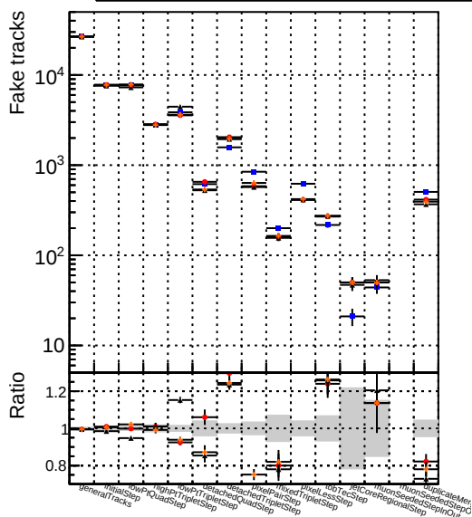
Number Model Dataset Model Model Model Model 1 DQM V0001 R0000000001 Global CMSSW mkFitPU50 RECO 2 DQM V0001 R0000000001 Global CMSSW mkFitPU50LowPtQuad RECO 3 DQM V0001 R0000000001 Global CMSSW mkFitPU50LowPtTriplet RECO
