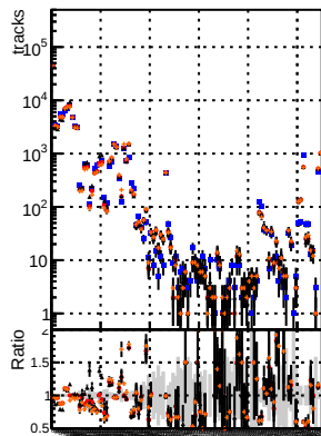
N of reco track vs. DQM V00001 R00000000001 Global CMS SSW mkFitPU50 LowPQuad RECO RECO
