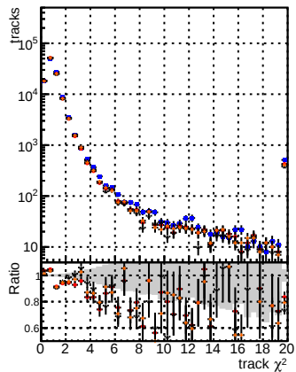
N of reco track vs. DQM V00001 R00000000001 Global CMS SSW mkFitPU50 LowPQuad RECO RECO
