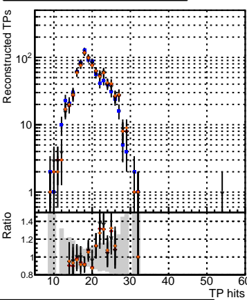
—●— DQM_V0001_R000000001_Global_CMSSW_ckfPU50_RECO —■— DQM_V0001_R000000001_Global_CMSSW_mkFitPU50_RECO —▲— DQM_V0001_R000000001_Global_CMSSW_mkFitPU50LowPtQuad_RECO —◆— DQM_V0001_R000000001_Global_CMSSW_mkFitPU50LowPtTriplet_RECO
