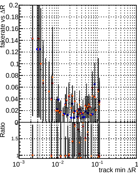
Fake rate vs \Delta R(\text{track}, \text{jet}) DQM V0001 R00000000001 Global CMSSW ch1PU50 RECO Global CMSSW ch1PU50 RECO Global CMSSW mktPU50 LowPQuad RECO Global CMSSW mktPU50 LowPTriplet RECO
