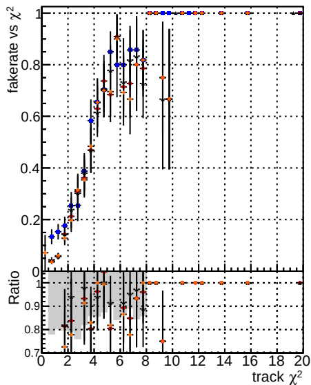
Fake rate vs. DQM V0001 B000000000001 Global CMSSW ckf RECO DQM V0001 R000000000001 Global CMSSW mkfit RECO DQM V0001 R000000000001 Global CMSSW mkfit LOWPQuad DQM V0001 R000000000001 Global CMSSW mkfit LowPtTriplet DQM V0001 R000000000001 Global CMSSW mkfit RECO
