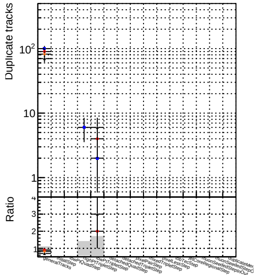
—●— DQM_V0001_R0000000001_Global_CMSSW_ckpt_RECO —◆— DQM_V0001_R0000000001_Global_CMSSW_mkfit_RECO —▲— DQM_V0001_R0000000001_Global_CMSSW_mkfitLowPtQuad_RECO —★— DQM_V0001_R0000000001_Global_CMSSW_mkfitLowPtTriplet_RECO
