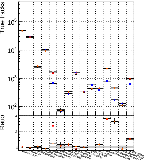
Number Color Label Model Fit Region Blue DQM V0001 R0000000001 Global CMSSW_ckpt_RECO Red DQM V0001 R0000000001 Global CMSSW_mkfit_RECO Black DQM V0001 R0000000001 Global CMSSW_mkfitLowPtQuad_RECO Orange DQM V0001 R0000000001 Global CMSSW_mkfitLowPtTriplet_RECO
