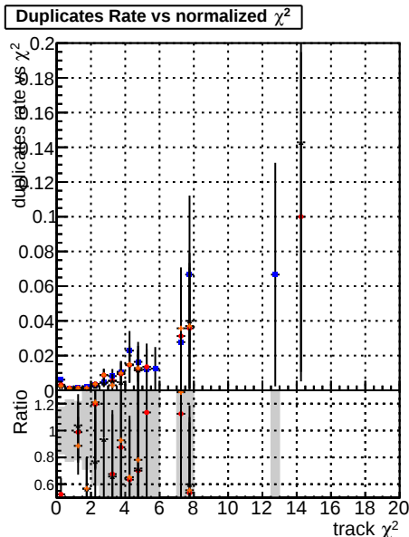
DOM V0001 R00000000001 Global CMSSW ekf RECO DOM V0001 R00000000001 Global CMSSW ekf RECO DOM V0001 R00000000001 Global CMSSW ekf RECO DOM V0001 R00000000001 Global CMSSW ekf RECO
