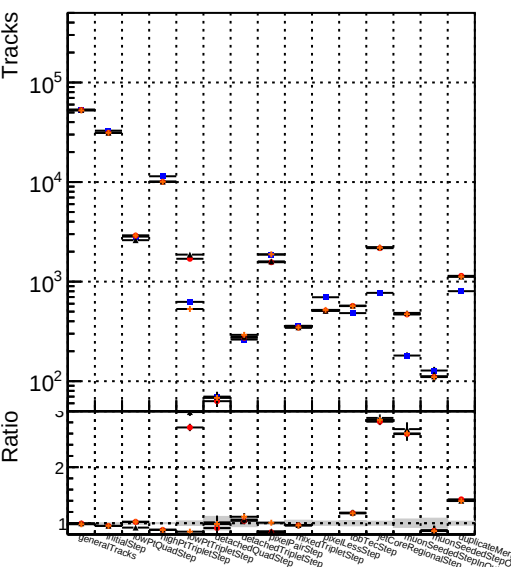
Number Symbol DQM V0001 R0000000001 Global CMSSW ckf RECO ● DQM V0001 R0000000001 Global CMSSW mkfit RECO ● DQM V0001 R0000000001 Global CMSSW mkfitLowPtQuad RECO ● DQM V0001 R0000000001 Global CMSSW mkfitLowPtTriplet RECO
