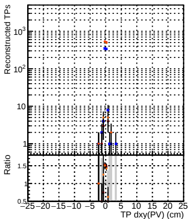
— DQM_V0001_R0000000001_Global_CMSSW_ckf_RECO — DQM_V0001_R0000000001_Global_CMSSW_mkfit_RECO — DQM_V0001_R0000000001_Global_CMSSW_mkfitLowPtQuad_RECO — DQM_V0001_R0000000001_Global_CMSSW_mkfitLowPtTriplet_RECO
