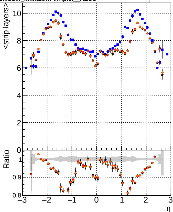
—■— DQM_V0001_R000000001 Global CMSSW_ckf_RECO —●— DQM_V0001_R000000001 Global CMSSW_mkfit_RECO —▲— DQM_V0001_R000000001 Global CMSSW_mkfitLowPtQuad_RECO —◆— DQM_V0001_R000000001 Global CMSSW_mkfitLowPtTriplet_RECO
