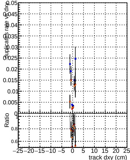
al-CMSSW-mkfit-LowPQuad-RECO al-CMSSW-mkfit-LowPTriplet-RECO
