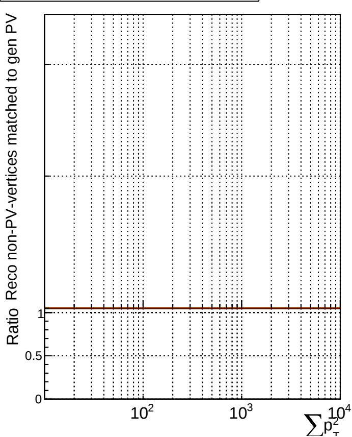
RecoAssoc2GenPVMatchedNotHighest_Pt2
