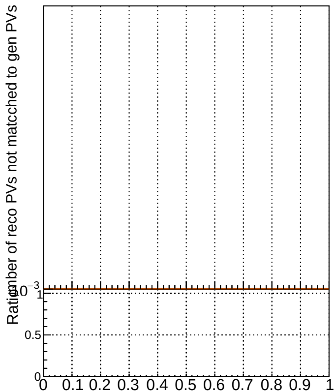
RecoPVAssoc2GenPVNotMatched_Purity
