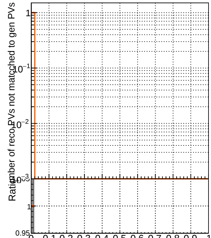
RecoPVAssoc2GenPVNotMatched_missing
