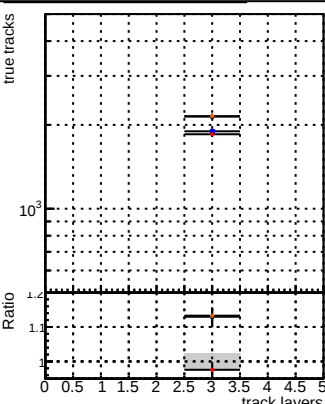
N of associated (recoToSim) tracks vs layer
