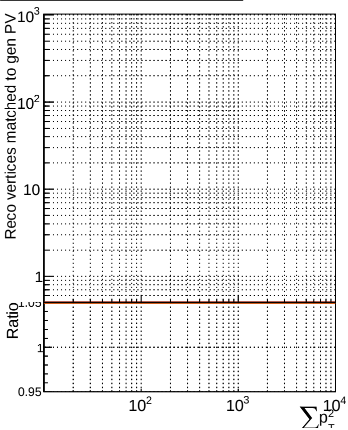
RecoAssoc2GenPVMatched_Pt2
