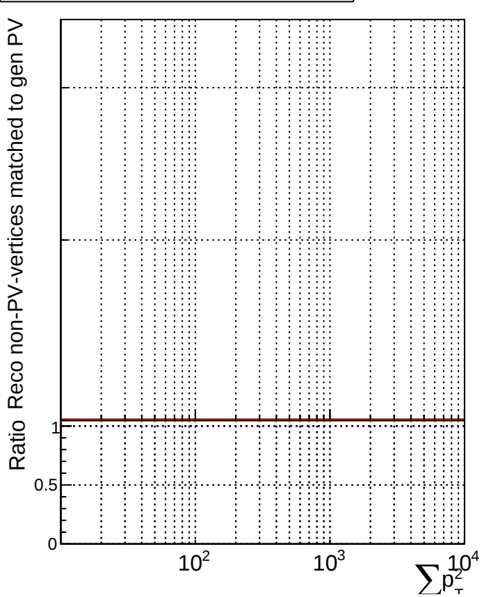
RecoAssoc2GenPVMatchedNotHighest_Pt2
